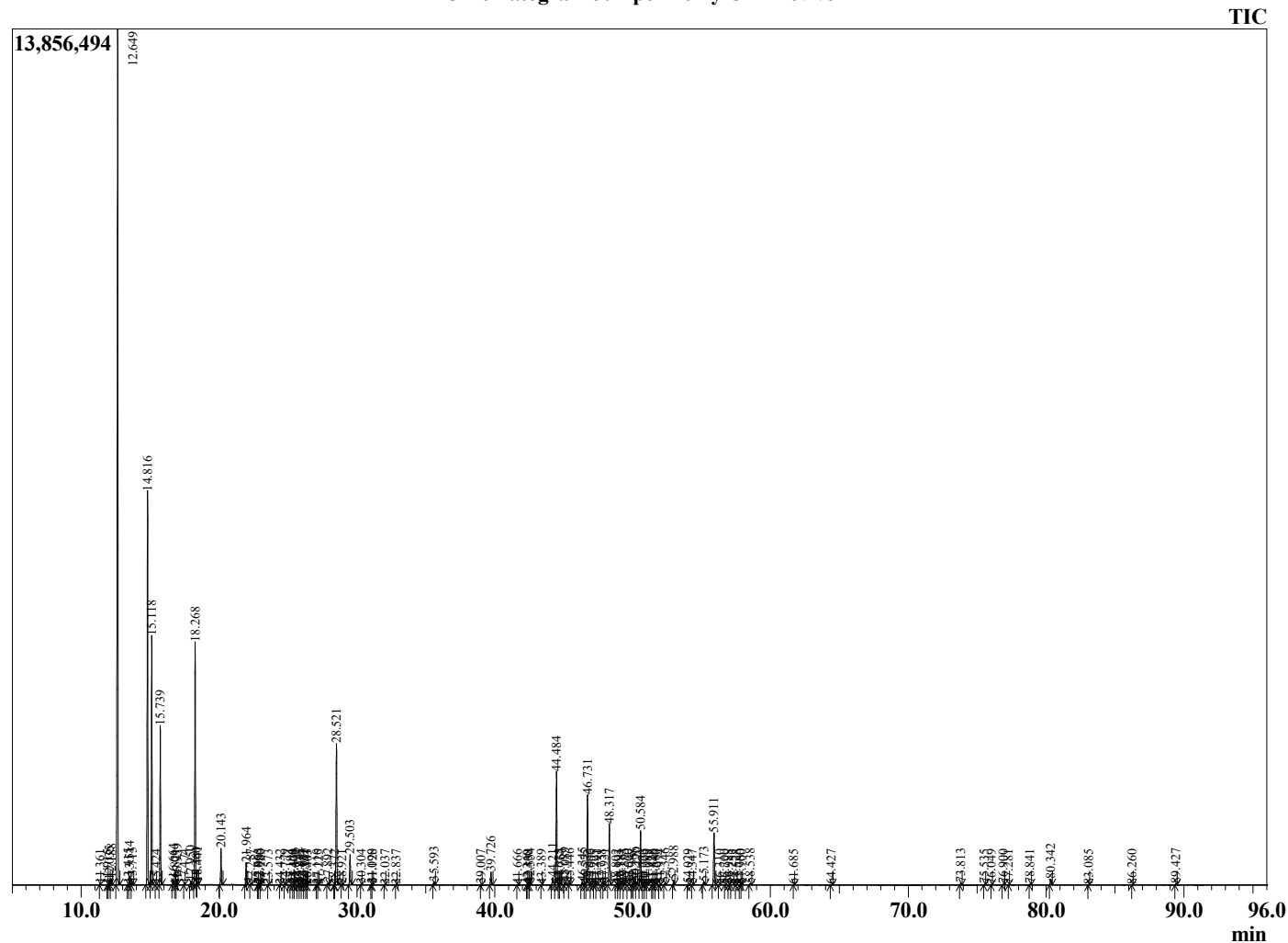
Chromatogram Juniper Berry Oil - Revive
