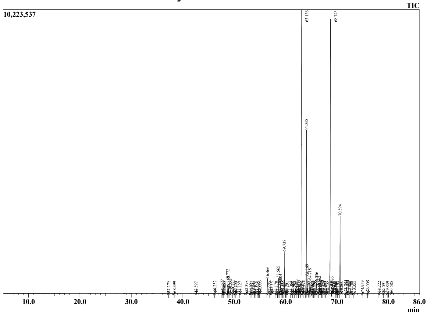
Chromatogram Buddha Wood Oil - Revive
