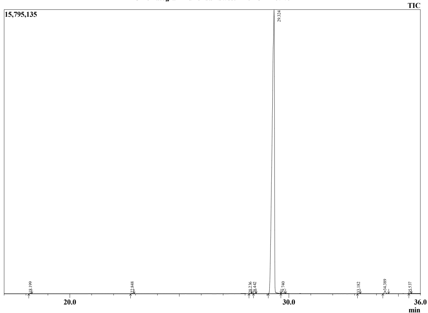
Chromatogram Adirondak Sweet Birch Oil- Revive
